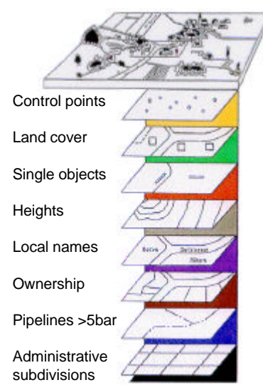
Figure 3: The 8 information layers of cadastral surveying.
